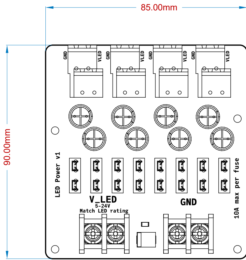
Top side component view (Scale 1:1)
