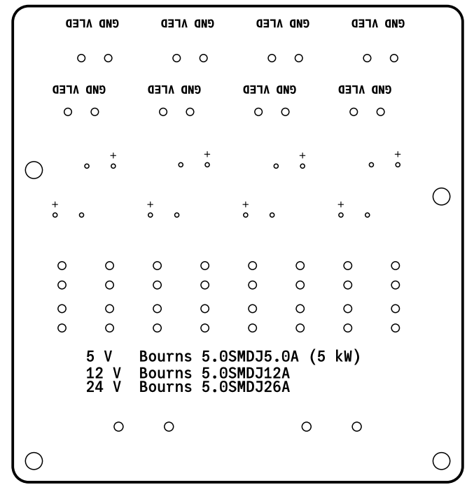
Bottom side component view (Scale 1:1)
