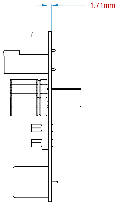
Right side component view (Scale 1:1)
